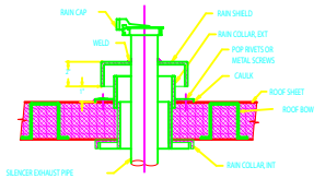
RAIN SHIELD / COLLAR INSTALLATION
